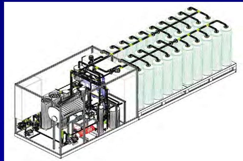
Plant Processing and Column View
